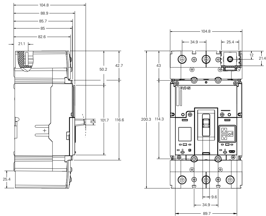
PDC2 circuit breaker, 3P
